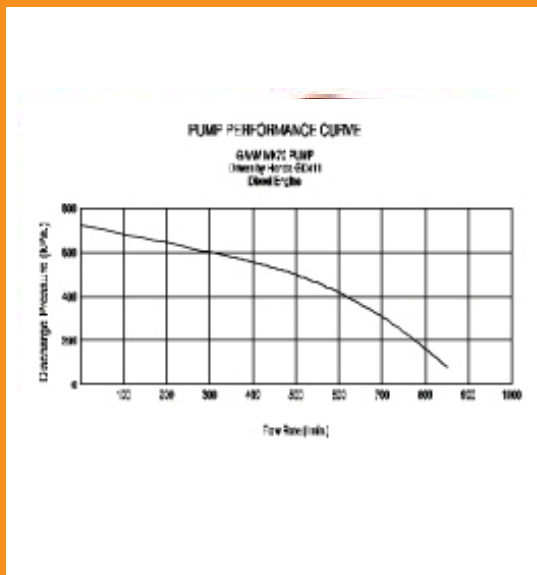
Pump performance curve
