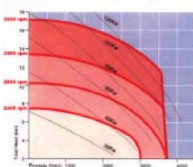
Typical high-pressure performance of Godiva World Series multi-pressure vehicle mounted pump range at 3m lift.
